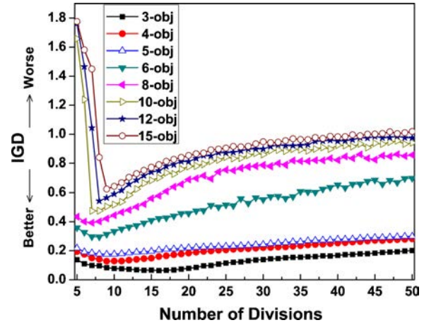
Fig. 6. IGD of GrEA with different numbers of divisions on DTLZ2.
